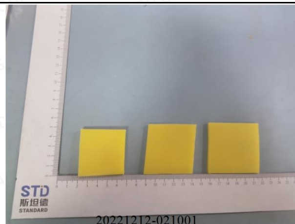
Fig.3. Photos of samples after the test of resistance to liquid chemical medium (5% H 2 SO 4 )
